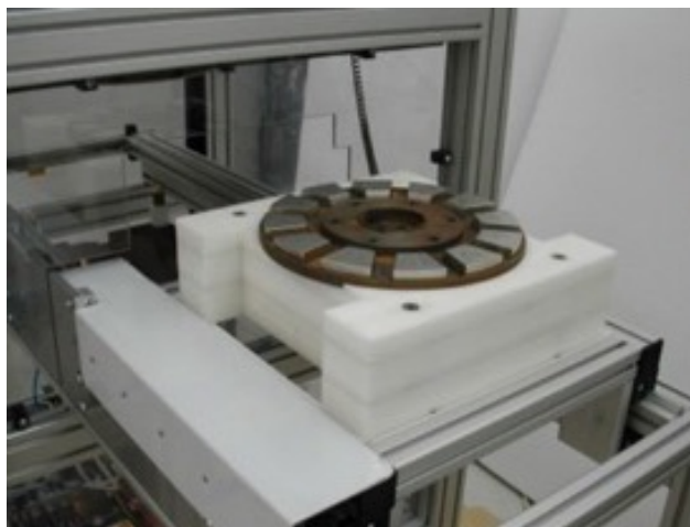
Custom Electric Motor fixture – Axial flux rotor (from 2005) being loaded into a production 12 pole custom fixture in a second-generation production tower M3000-80kj.
